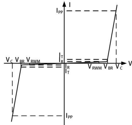
Bi-Directional TVS
